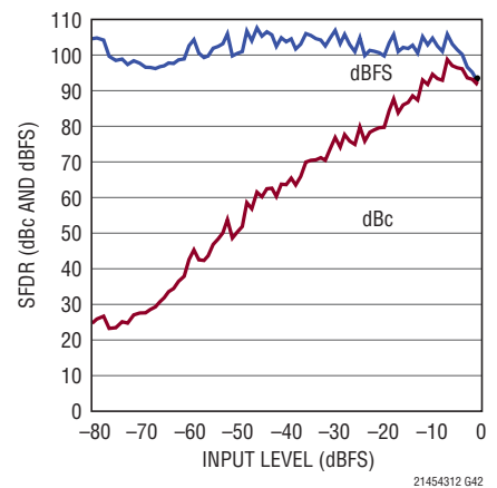
LTC2143-12: SFDR vs Input Level, f_{IN} = 70\text{MHz} , 80\text{Mpsps} , 2\text{V} Range
