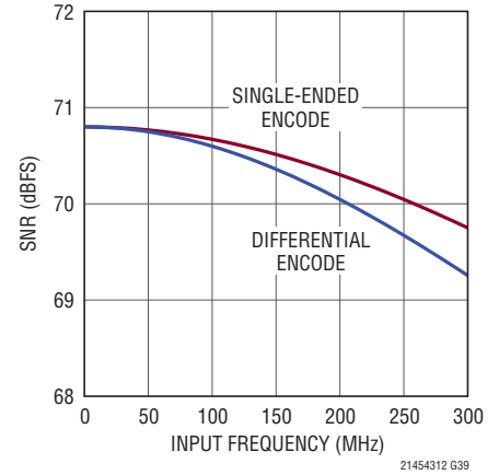
LTC2143-12: SNR vs Input Frequency, -1\text{dBFS} , 80\text{Mpsps} , 2\text{V} Range
