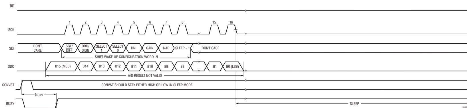
Figure 10. Sleep Mode Operation for the LTC1859*
