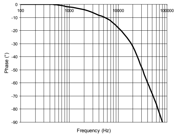
HAH1DR 700 Phase
