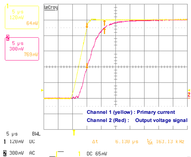
Typical response time at 100 A/
