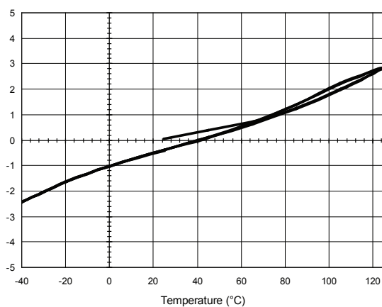
HAH1BV S/20 Gain Error (%)
