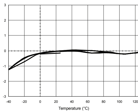
HAH1BV S/20 Electrical offset Error (A)
