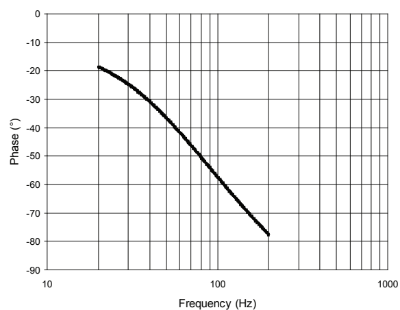
HAH1BV S/20 Phase
