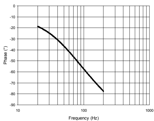
HAH1BV S/18 Phase
