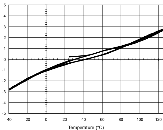
HAH1BV S/18 Gain Error (%)
