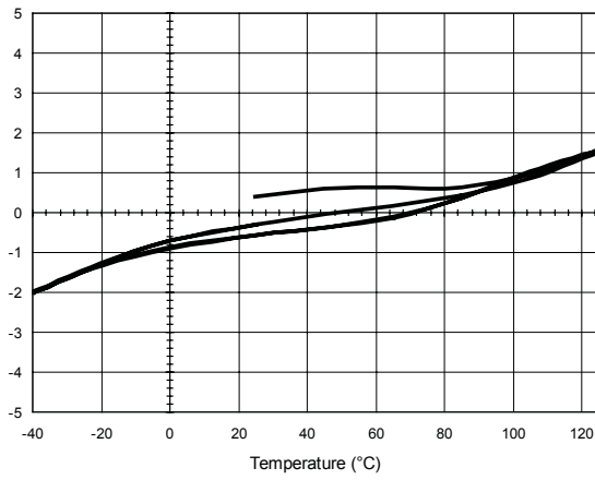
HAH1BV S/07 Gain Error (%)
