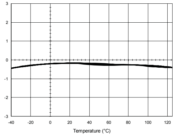
HAH1BV S/07 Electrical offset Error (A)
