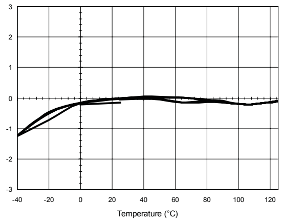
HAH1BV S/04 Electrical offset Error (A)
