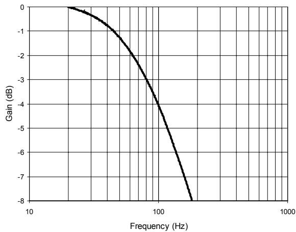
HAH1BV S/04 Frequency Bandwidth
