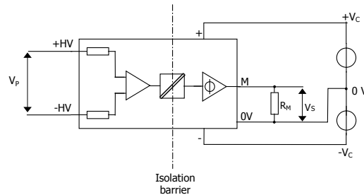
Figure 17: standard characterization schematics for voltage output transducers ( R_M = 100 \text{ k}\Omega unless otherwise noted)
