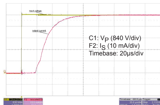
Figure 6: Typical step response (0 to 4200 V)
