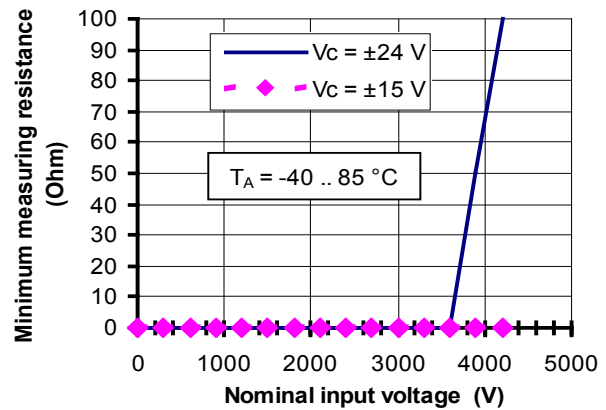
Figure 2: Minimum measuring resistance Under T_A = 80 \text{ }^{\circ}\text{C} , the minimum measuring resistance is 0 whatever V_C
