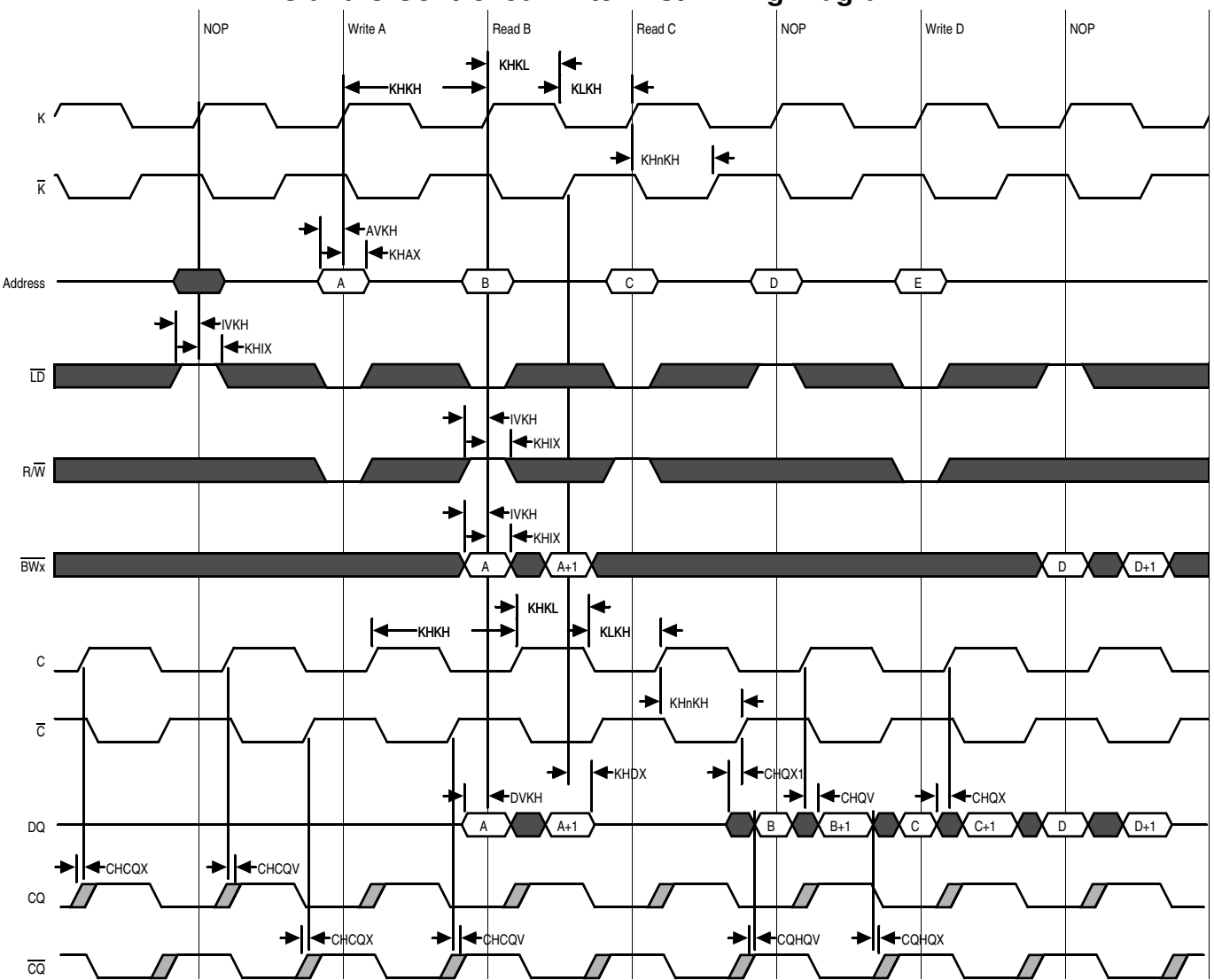
C and \bar{C} Controlled Write First Timing Diagram
