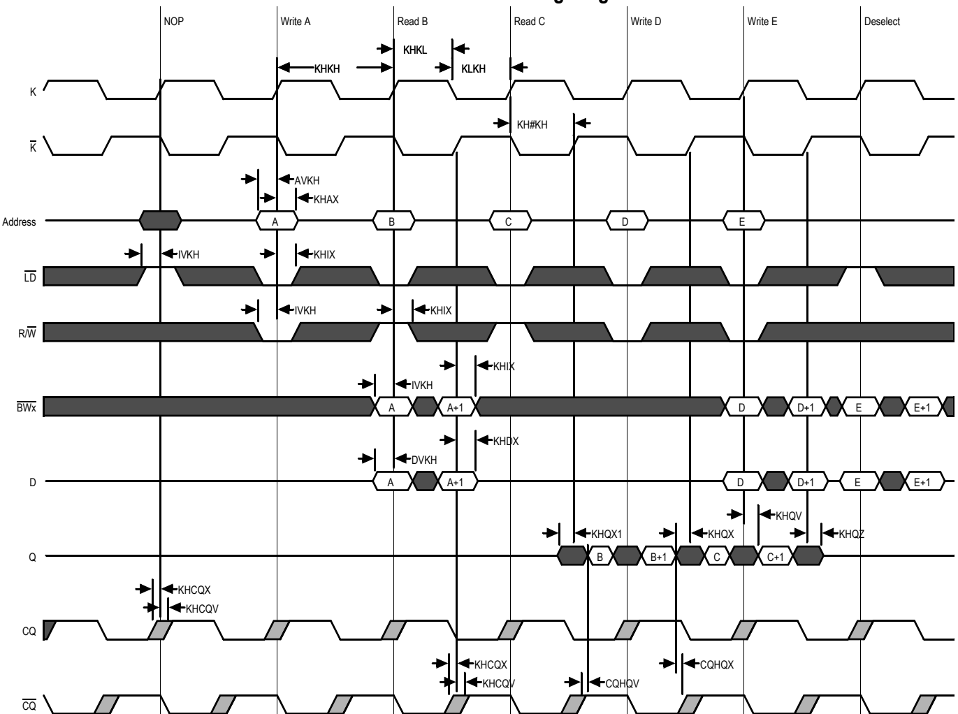
K Controlled Write-First Timing Diagram
