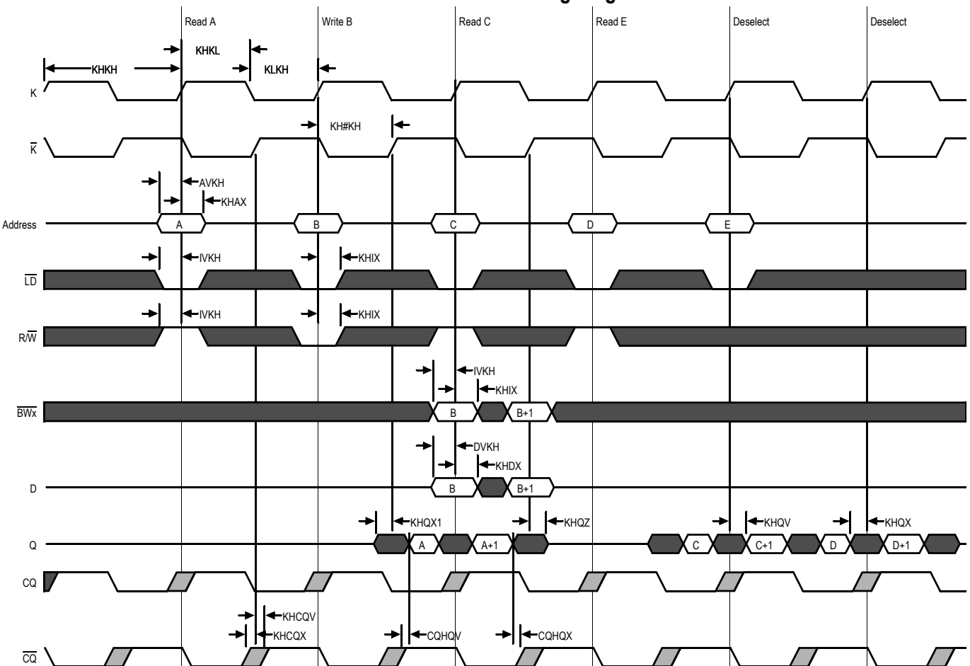
K Controlled Read-First Timing Diagram
