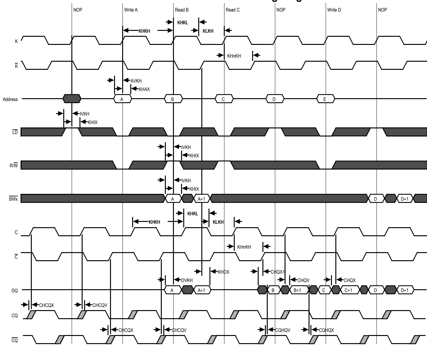
C and \overline{C} Controlled Write First Timing Diagram
