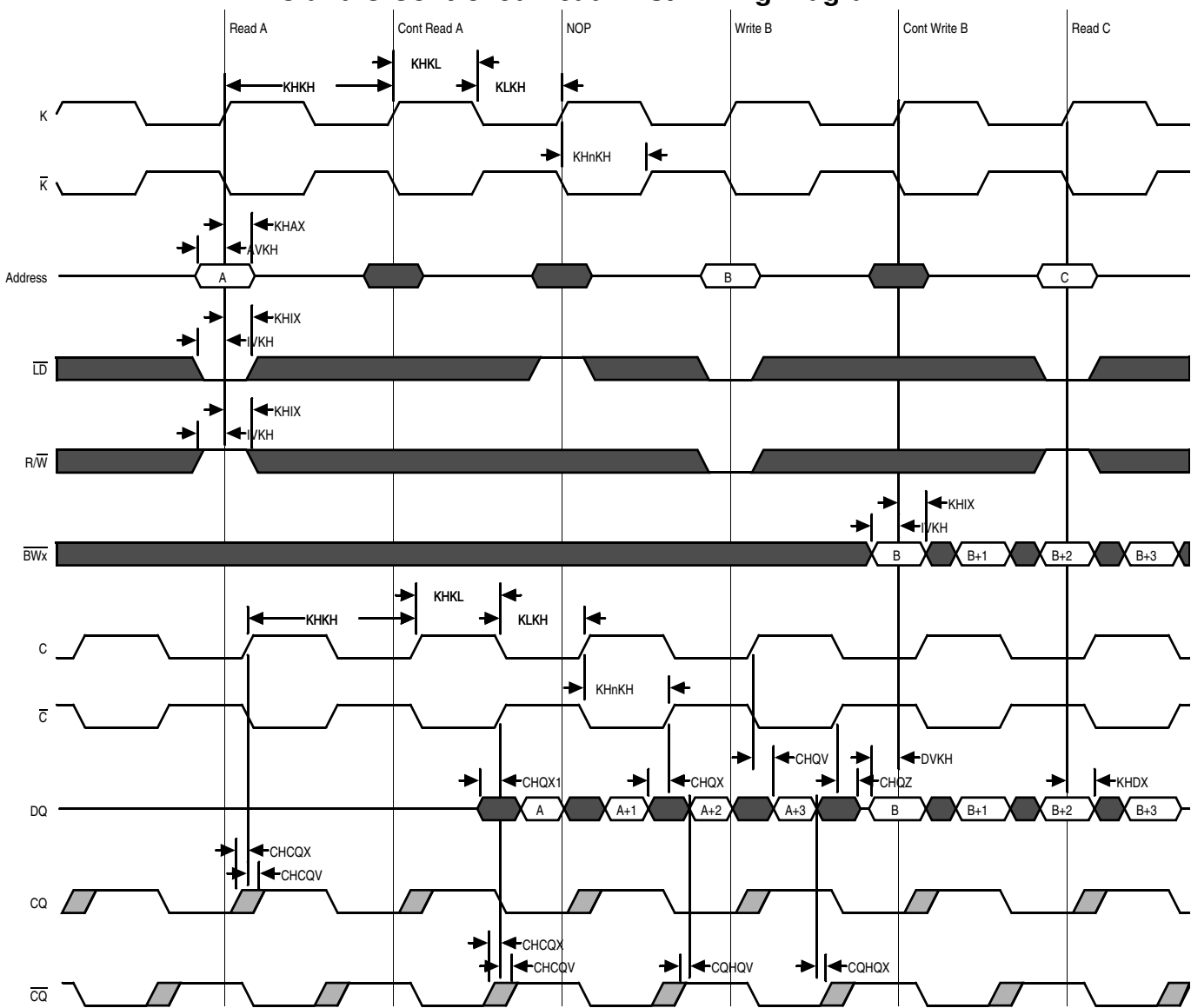
C and \bar{C} Controlled Read First Timing Diagram
