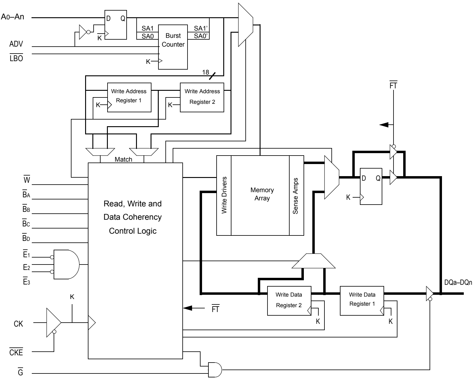
GS8321Z18/32/36E-xxxV NBT SRAM Functional Block Diagram
