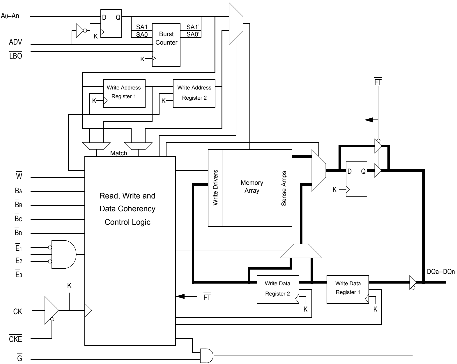
GS8320Z18/36T-xxxV NBT SRAM Functional Block Diagram
