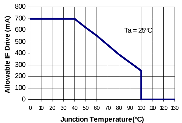
Derating Curve/die
