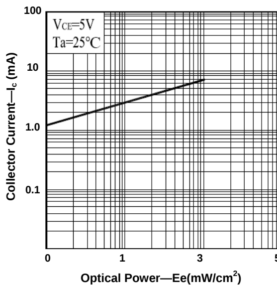
Collector Current— I_C (mA) vs Optical Power— E_e (mW/cm 2 )
