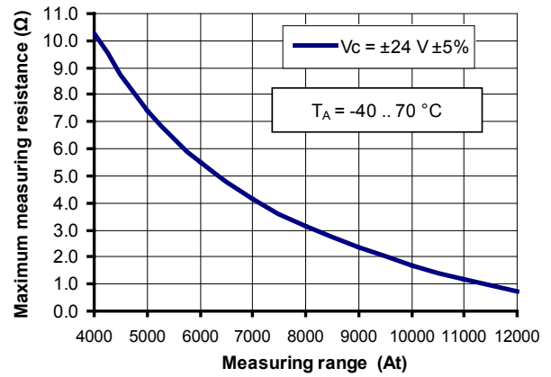
Figure 2: R_M for ranges 4000 .. 12000 A
