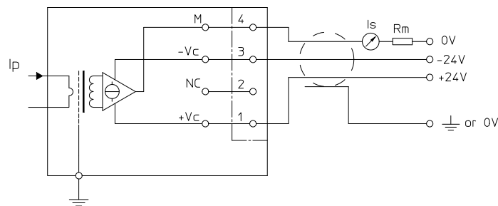
Figure 5: Connection principle
