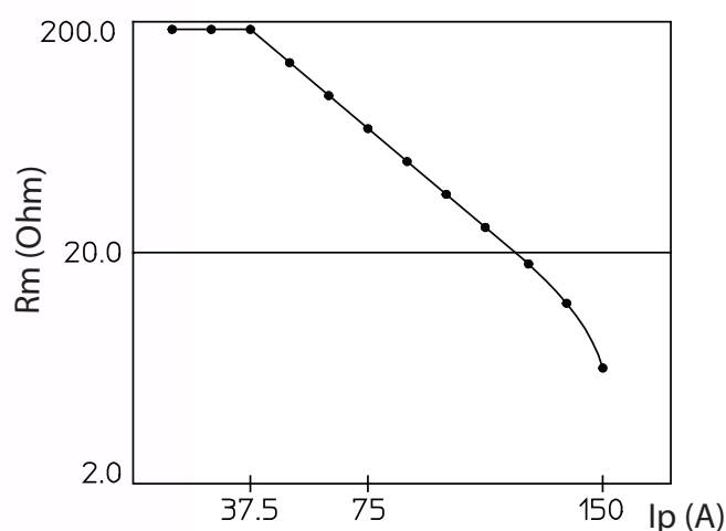
Measuring resistor vs primary current
