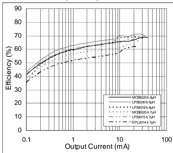
Figure 37. Efficiency Comparison of different Inductors; V IN = 3V, V OUT = 18V
