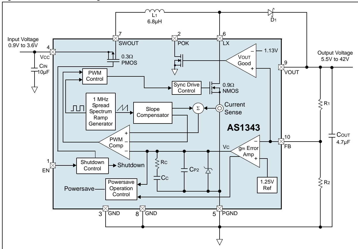
Figure 27. AS1343 - Block Diagram with Shutdown Disconnect Switch
