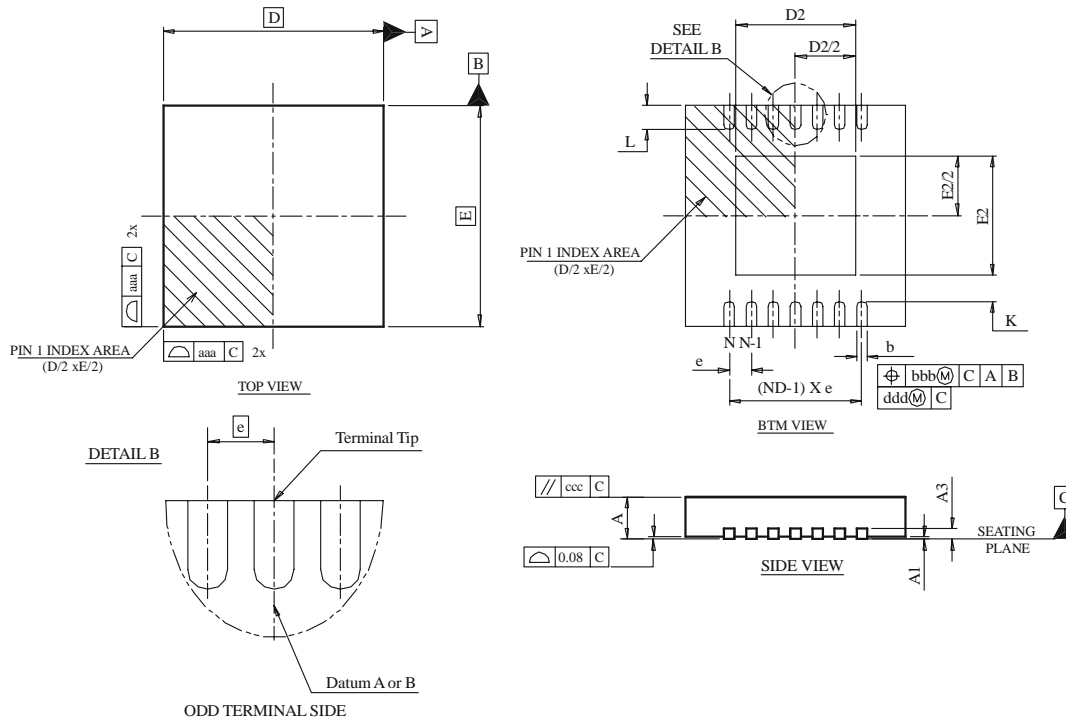
Figure 34. TDFN-10 3x3mm Package
