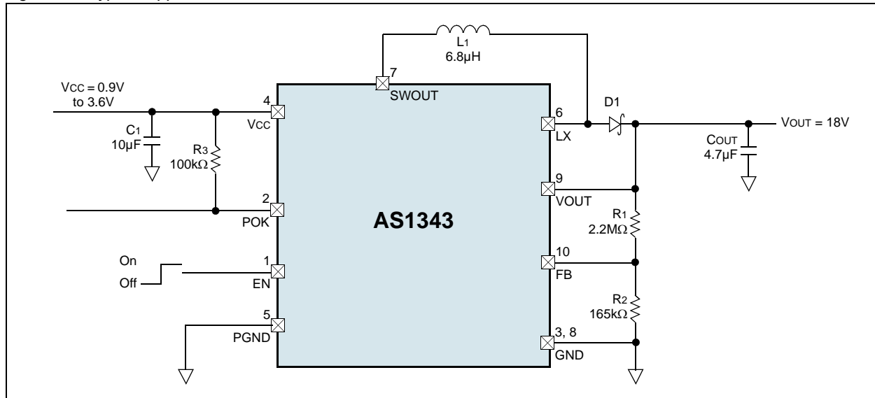
Figure 28. Typical Application
