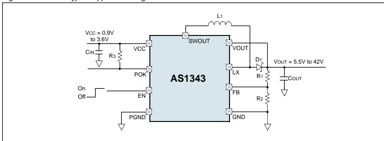
Figure 1. AS1343 - Typical Application Diagram
