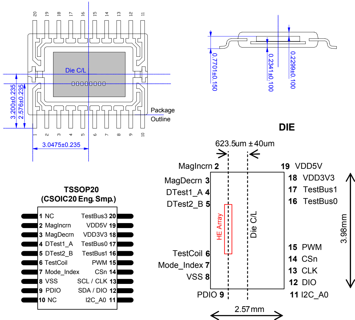
Figure 14. 20-pin TSSOP Package
