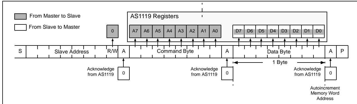
Figure 18. Command and Single Data Byte received by AS1119
