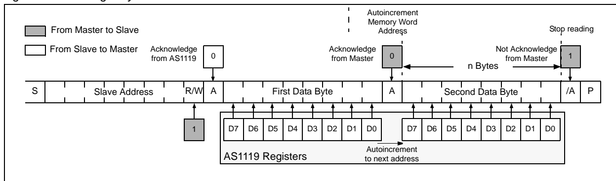
Figure 20. Reading n Bytes from AS1119
