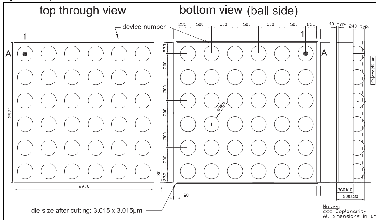
Figure 24. 36-pin WL-CSP
