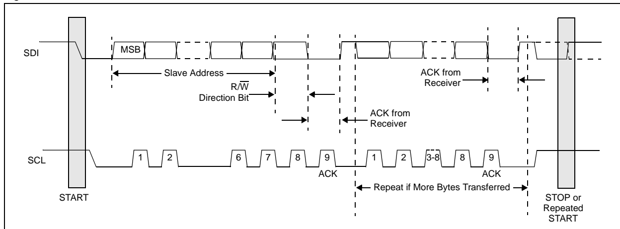
Figure 15. Bus Protocol
