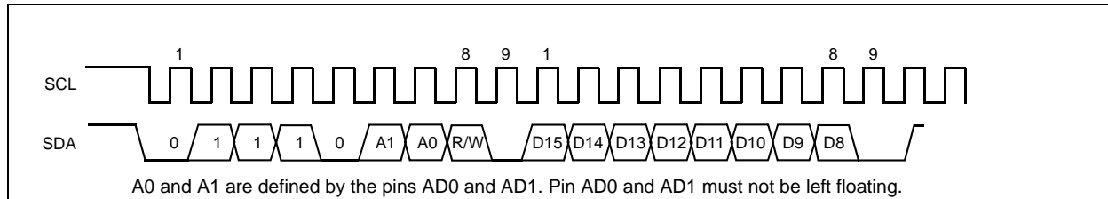
Figure 14. I 2 C Interface Initialisation
