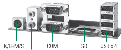
▲ I/O board
