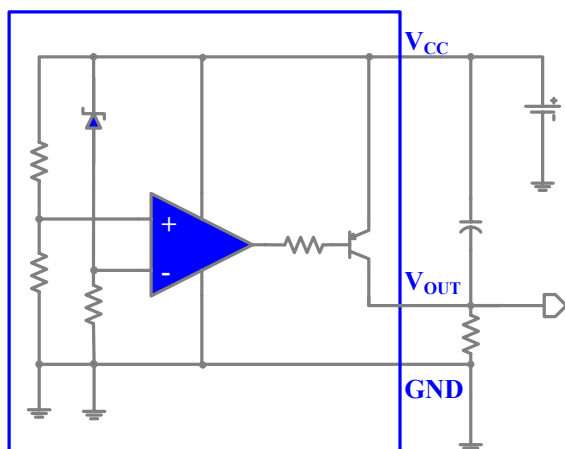
Test Circuit 1
