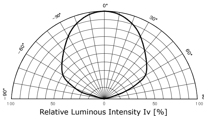
Fig. 5 Radiation Diagram
