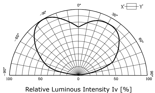
Fig. 5-2 Radiation Diagram(Y)
