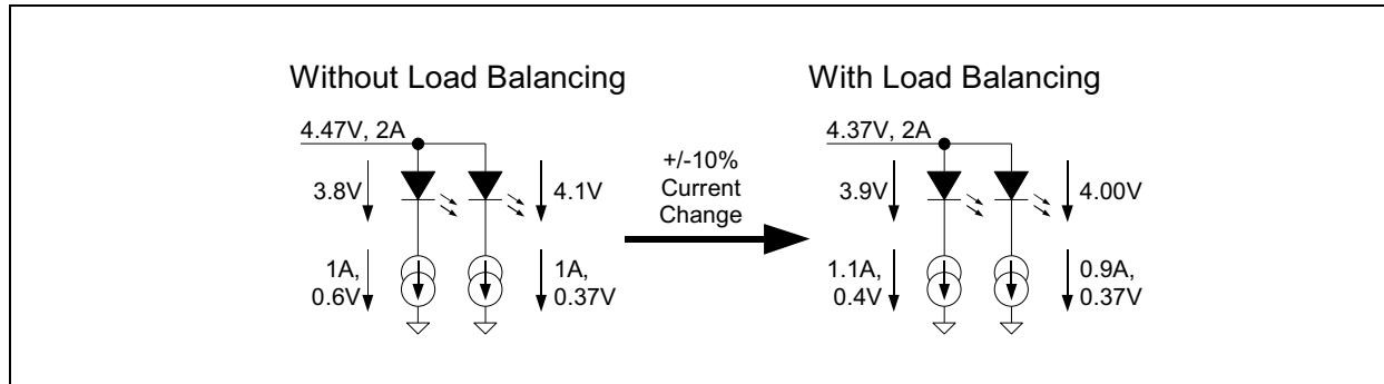
Figure 23. Load Balancing
