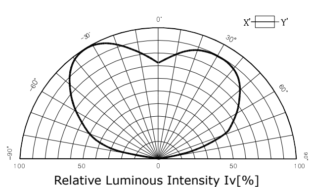
Fig. 5-2 Radiation Diagram(Y)
