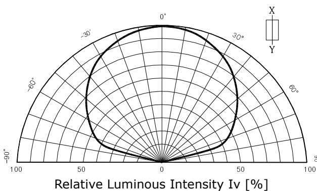
Fig. 5-1 Radiation Diagram(X)
