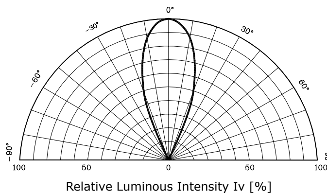
Fig. 5 Radiation Diagram
