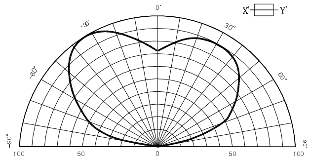
Fig. 5-2 Radiation Diagram(Y)
