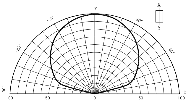
Fig. 5-1 Radiation Diagram(X)
