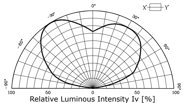
Fig. 5-2 Radiation Diagram(Y)
