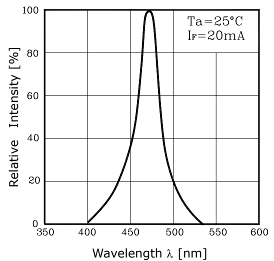
Fig.4 Spectrum Distribution
