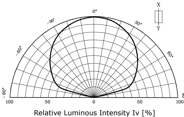
Fig. 5-1 Radiation Diagram(X)
