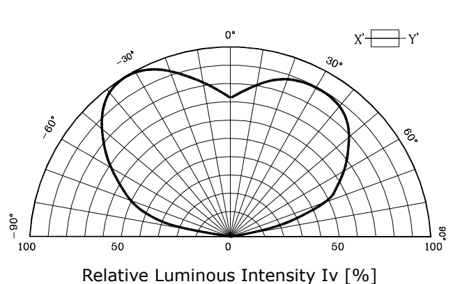
Fig. 5-2 Radiation Diagram(Y)
