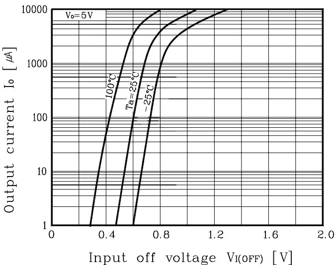
Fig. 2 I_O - V_{I(OFF)}
