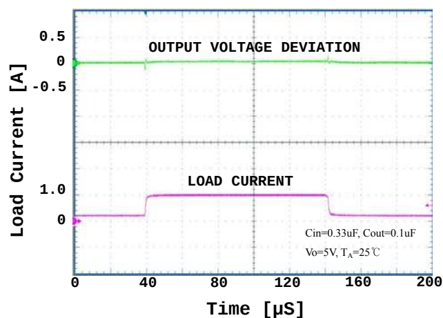
Fig.6 Load Transient Response
