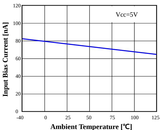
Fig.4 Input Bias Current vs. Ambient Temp.
