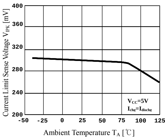
Fig.5 T_A vs. V_{IPK(sense)}
