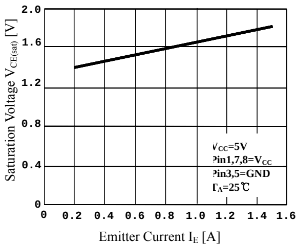
Fig.3 I_E vs. V_{CE(sat)}
