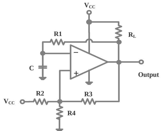
Square-wave Oscillator
