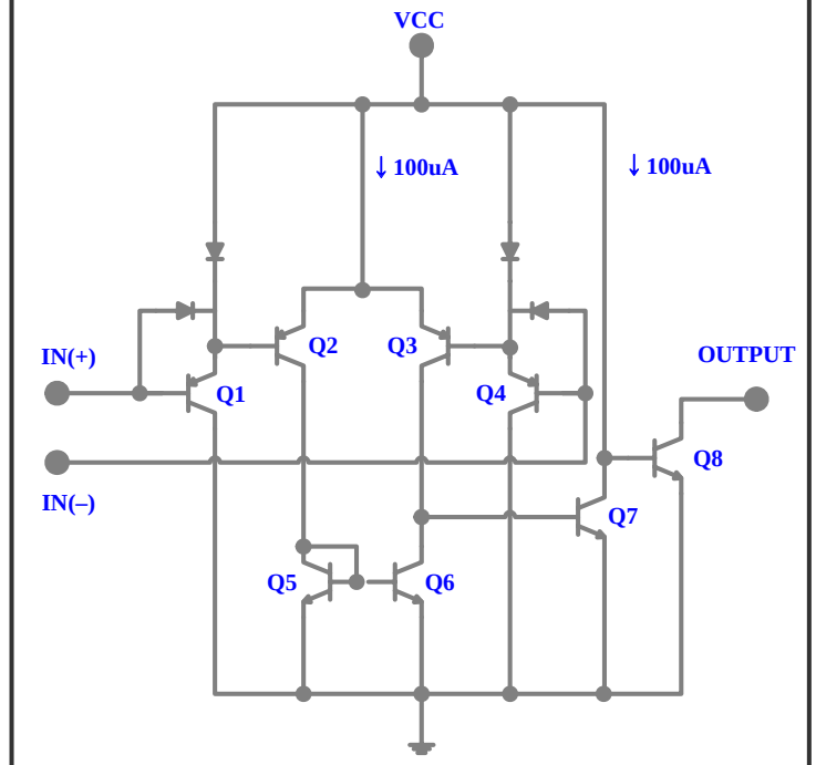
Equivalent Circuit
