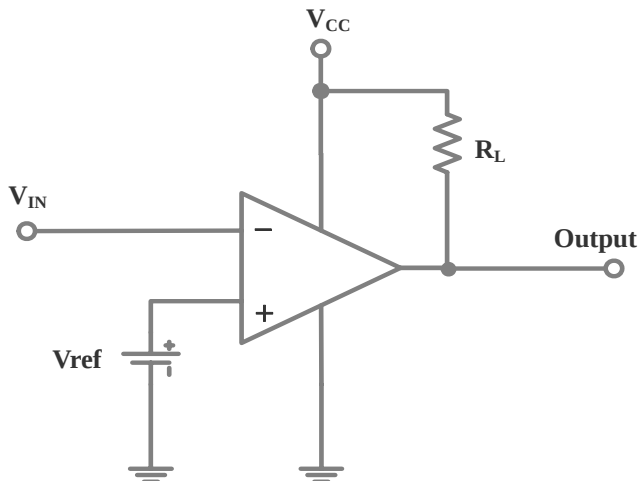
Basic Comparator
