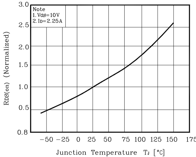
Fig. 8 R_{DS(on)} - T_J
