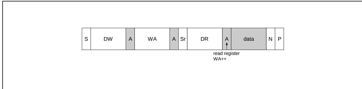
Figure 23. Random Read
