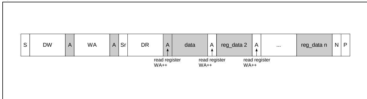
Figure 24. Sequential Read
