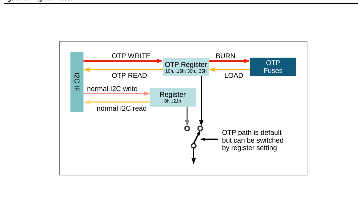
Figure 19. Register Access
