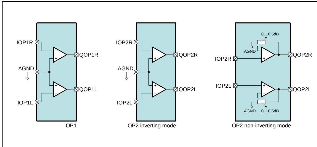
Figure 16. Operational Amplifiers
