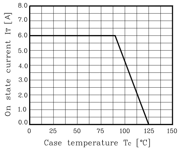
Fig. 2 I_{T(RMS)} - T_C
