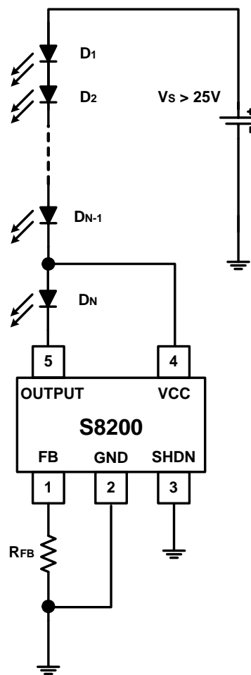
<APP5. High Voltage Operation of S8200 (2) >
