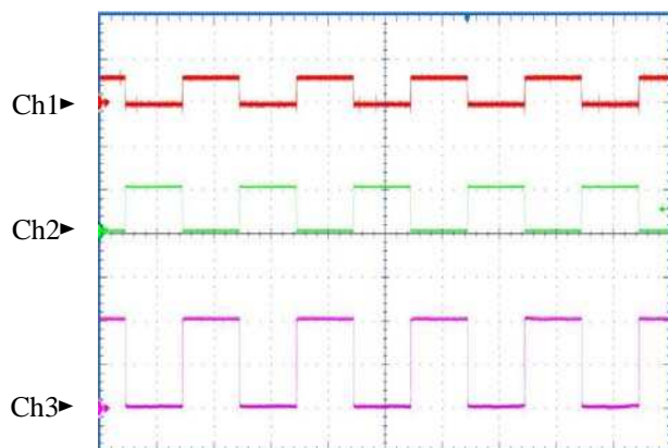
Fig.7 Dimming Waveform
