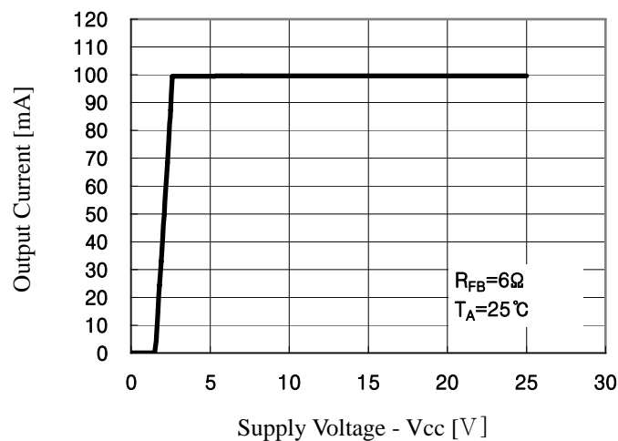
Fig.6 Output Current vs Supply Voltage
