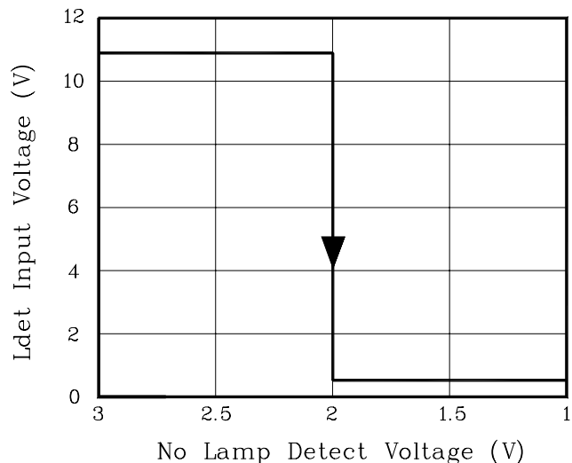
Fig. 4 Ldet Input Voltage vs. No Lamp Detect Voltage
