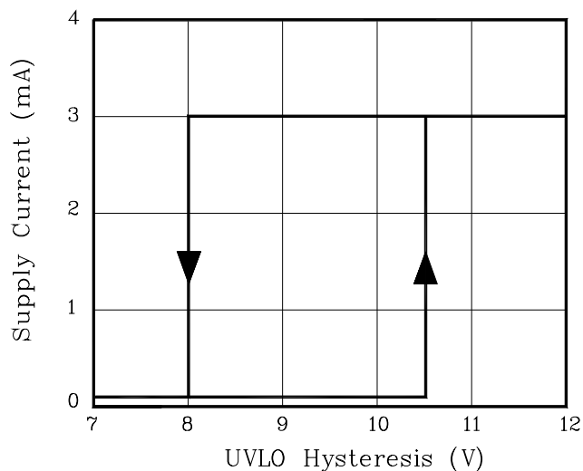
Fig. 3 Supply Current vs. UVLO Hysteresis
