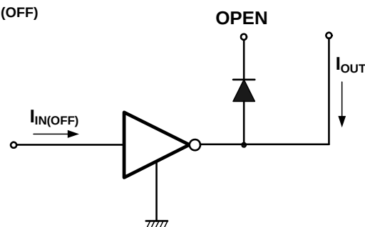
4. I_{IN(OFF)}
