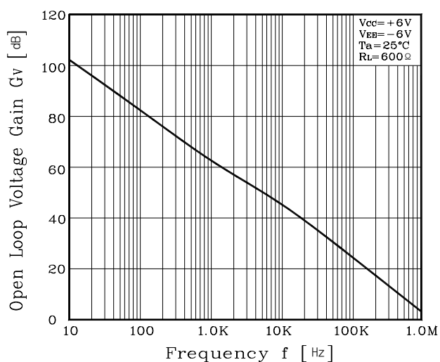
Fig. 8 G_V vs f
