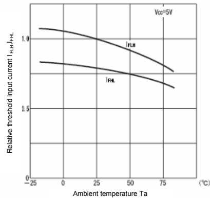
Relative threshold input current Vs. Ambient temperature
