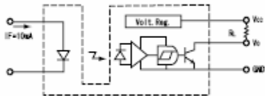
Measurement of high level output voltage
