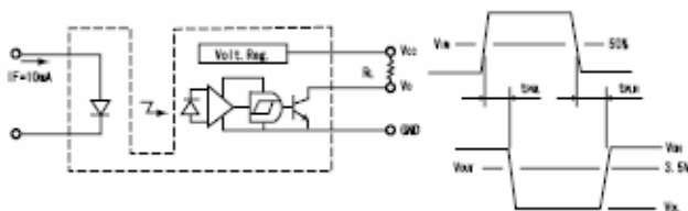
Measurement of propagation time
