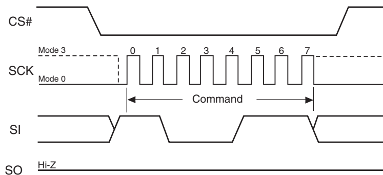
Figure 9.11 Bulk Erase (BE) Command Sequence
